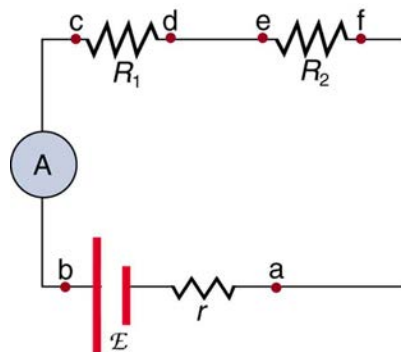
Figure 21.28 An ammeter ( A ) is placed in series to measure current. All of the current in this circuit flows through the meter. The ammeter would have the same reading if located between points d and e or between points f and a as it does in the position shown. (Note that the script capital E stands for emf, and r stands for the internal resistance of the source of potential difference.)
