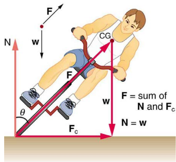
Figure 6.36 A bicyclist negotiating a turn on level ground must lean at the correct angle—the ability to do this becomes instinctive. The force of the ground on the wheel needs to be on a line through the center of gravity. The net external force on the system is the centripetal force. The vertical component of the force on the wheel cancels the weight of the system while its horizontal component must supply the centripetal force. This process produces a relationship among the angle \theta , the speed v , and the radius of curvature r of the turn similar to that for the ideal banking of roadways.
